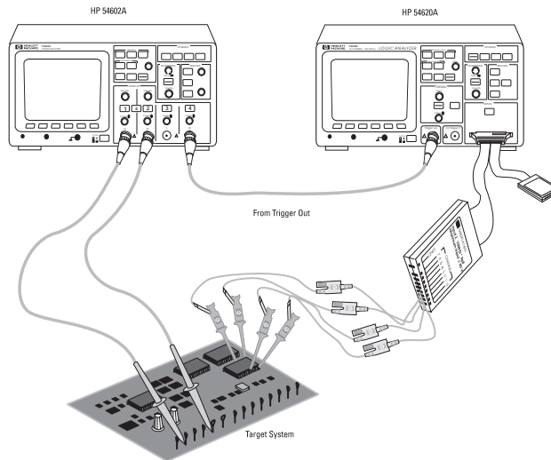
Connections for Triggering an Oscilloscope
