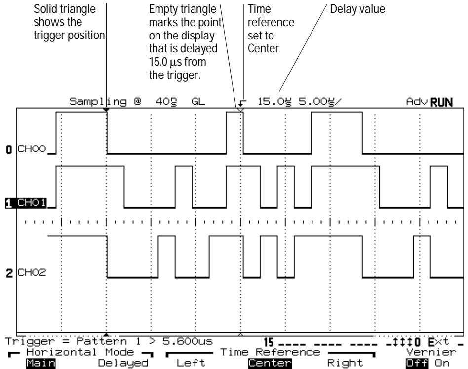
Time Reference at Center, Delay of 15 \mu\text{s} on Main Sweep
